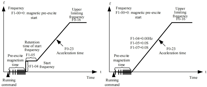
Figure 4-12. Schematic Diagram of Pre-excitation Start-up
