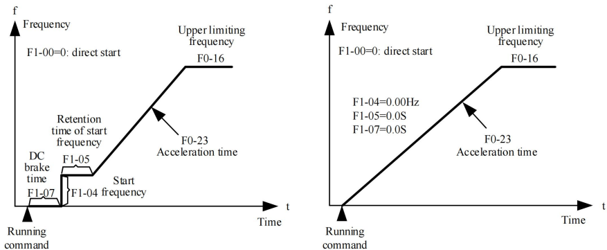
Figure 4-11. Schematic Diagram of Direct Start-up
