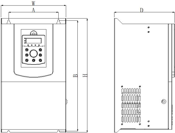
Figure 2-4. 380V(4T) 18~37kW Sheet Metal Chassis External and Installation Dimensions Diagram
