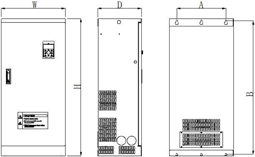
Figure 2-6. 380V(4T) 160~450kW VFD External and Installation Dimensions Diagram 660V(7T) 75~450kW VFD External and Installation Dimensions Diagram
