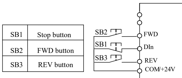
Figure 5-9. Three-wire Operation Mode I
