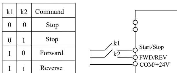
Figure 5-8. Two-line Operation Mode II
