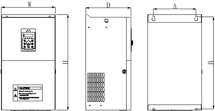
Figure 2-5. 380V(4T) 45~132kW VFD External and Installation Dimensions Diagram 660V(7T) 30~55kW VFD External and Installation Dimensions Diagram
