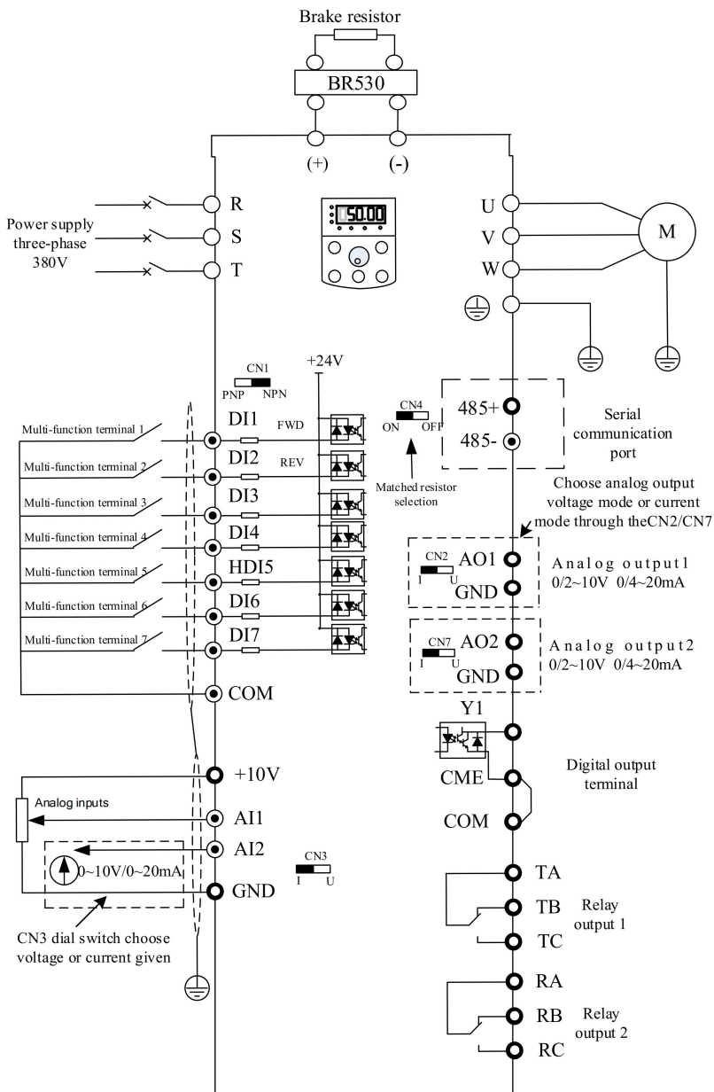
Figure 3-7. (4T/7T)37kW ~ 55kW Three-phase VFD
