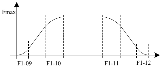
Figure 5-3. S-curve Acceleration and Deceleration Diagram
