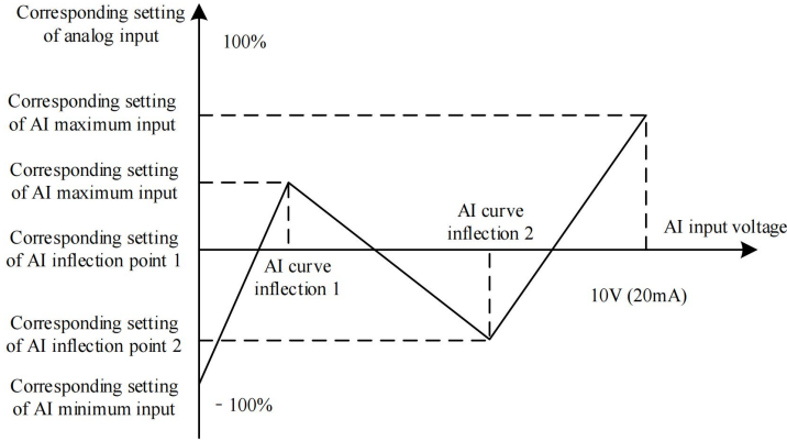
Figure 5-30 Schematic Diagram of Multi-point Curve
