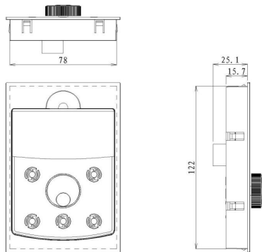
Figure 2-10. Installation Dimension Diagram of External Keyboard with Tray
