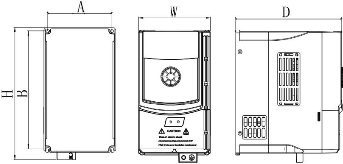
Figure 2-3. Schematic Diagram of the External Dimensions and Installation Dimensions of the Plastic Case Chassis Below 220V (3S) 2.2kW
