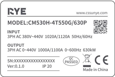
Figure 2-2. Nameplate
