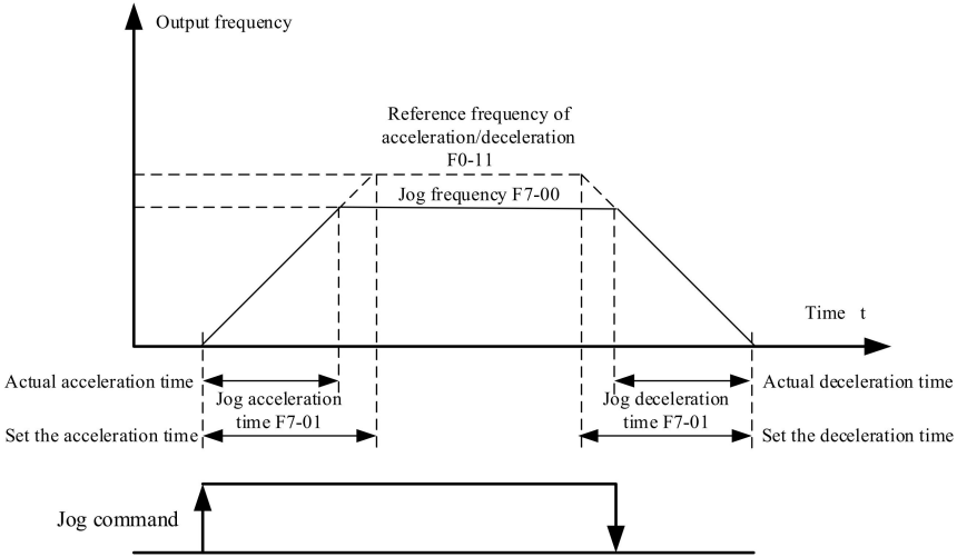
Figure 4-14. Inching Operation Diagram
