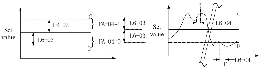
Figure 5-33. Wake up Diagram
