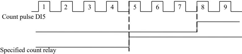
Figure 5-27. Schematic Diagram of Setting Count Value Setting and Specified Count Value Setting
