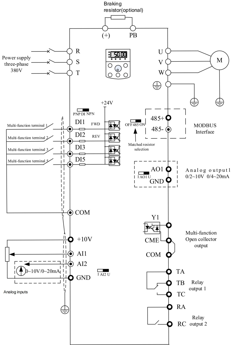
Figure 3-5. Three-phase VFD Below 2.2kW
