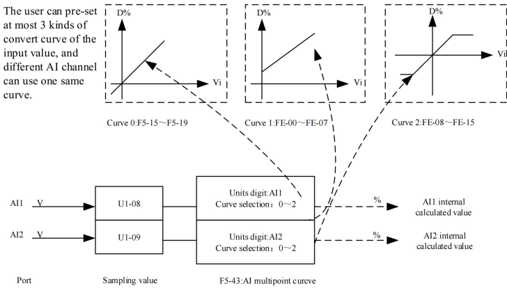
Figure 4-28. Correspondence Between AI Signals and Actual Settings
