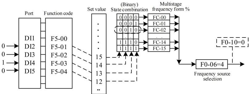
Figure 4-21. Multi-speed Control Diagram
