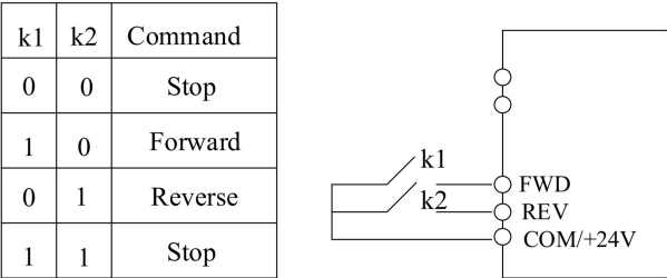
Figure 5-7. Two-line Operation Mode I
