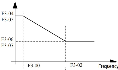
Figure 5-6. Schematic Diagram of Speed Loop PI Parameter Switching
