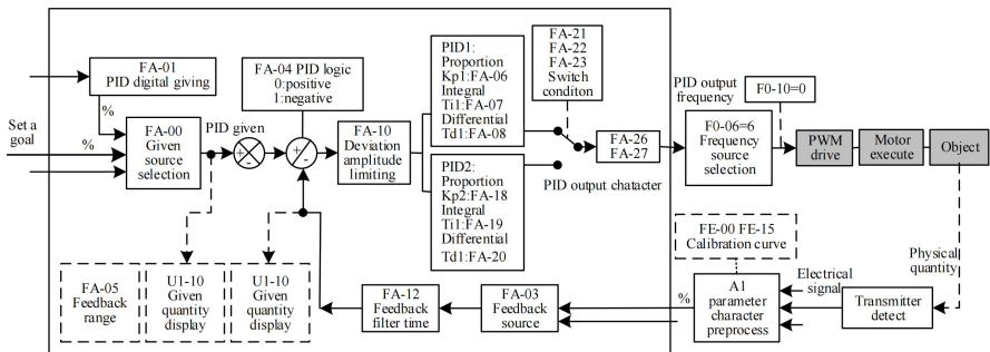
Figure 4-19. Schematic Diagram of Frequency Closed-loop Control
