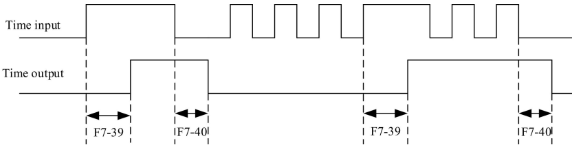
Figure 5-19. Timer Input/Output Action Diagram
