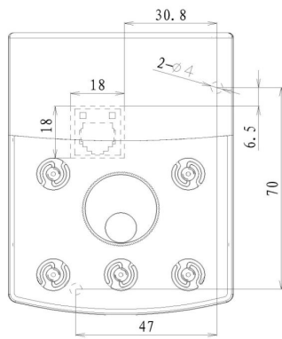
Figure 2-11. Installation Dimension Diagram of External Keyboard Without Tray
