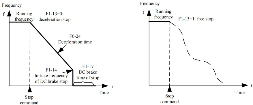
Figure 4-13. Shutdown Diagram
