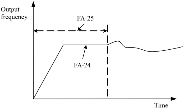
Figure 5-25. Schematic Diagram of PID Initial Value Function
