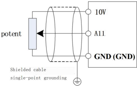
Figure 3-9. Schematic Diagram of Analog Input Terminal Wiring
