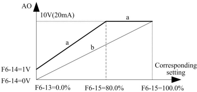
Figure 4-29. AO Output Diagram
