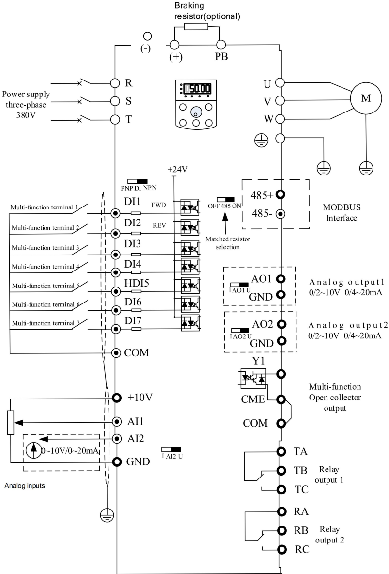
Figure 3-6. (4T/7T) Three-phase VFD Below 30kW
