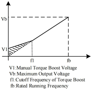
Figure 5-4. Manual Torque Lifting Diagram
