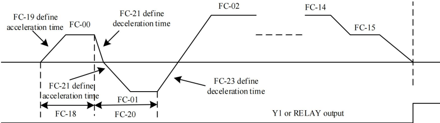
Figure 5-28 Simple PLC Diagram
