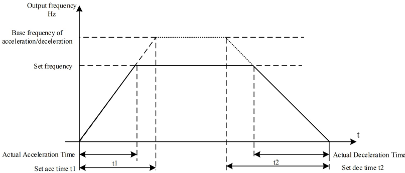
Figure 5-2. Schematic Diagram of Acceleration and Deceleration Time
