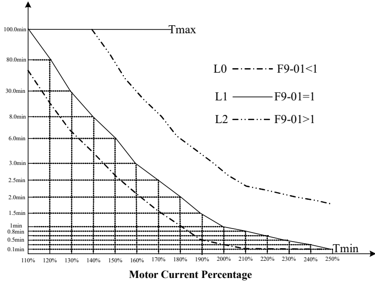
Figure 5-21 Overload Protection Curve of Motor
