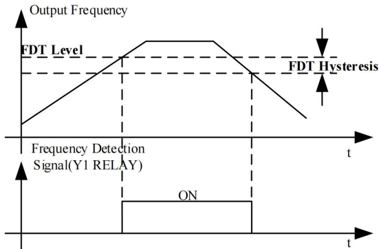
Figure 5-15. FDT Level Diagram
