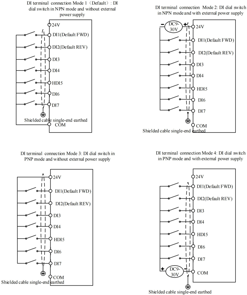
Figure 3-10. Wiring Diagram of Digital Input Terminals in Four Different Modes
