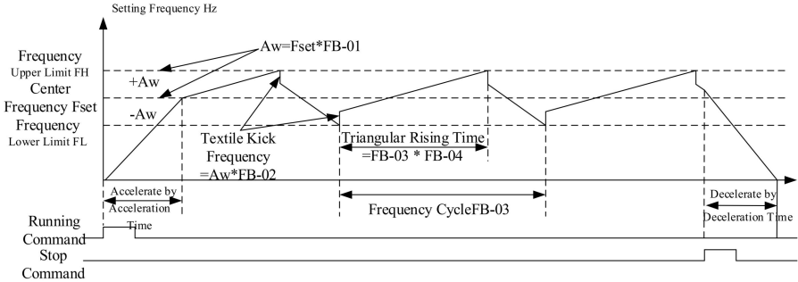
Figure 5-26 Schematic Diagram of Swing Frequency Operation
