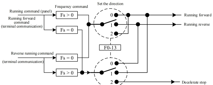
Figure 4-22. Schematic Diagram of Motor Running Direction
