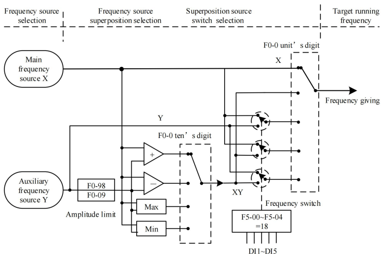
Figure 5-1. Schematic Diagram of Frequency Source Superposition
