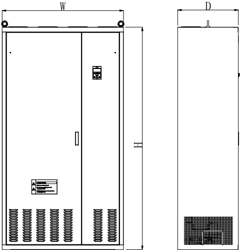
Figure 2-7. 380V(4T) 500~800kW VFD External and Installation Dimensions Diagram 660V(7T) 500~710kW VFD External and Installation Dimensions Diagram
