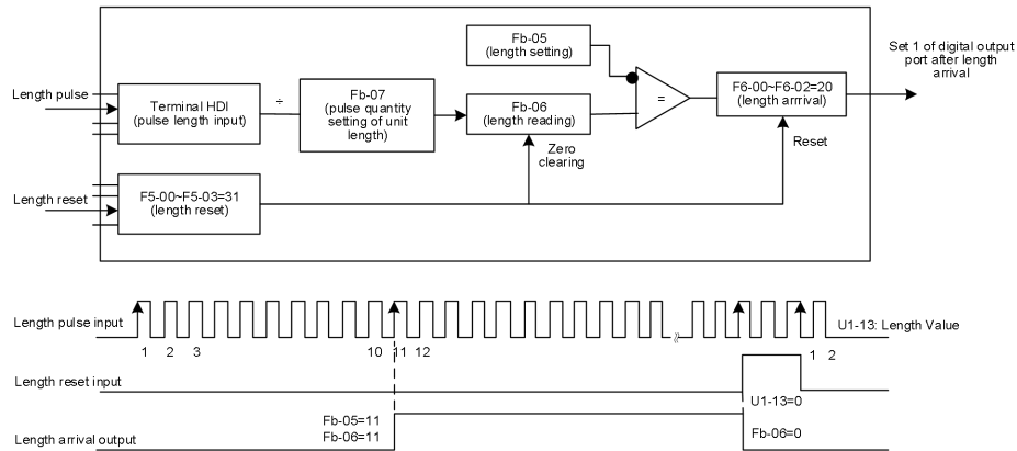
Fig.3-14 Function code setting of fixed-length control mode
