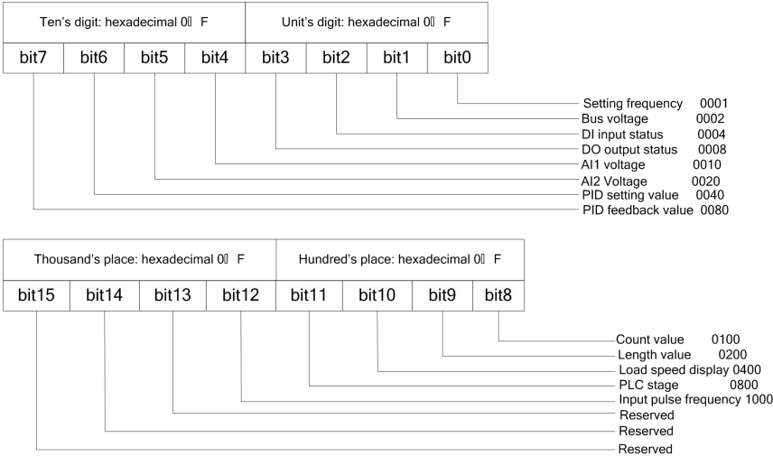
Fig.3-19 LED stop display3 F7-30 illustration
