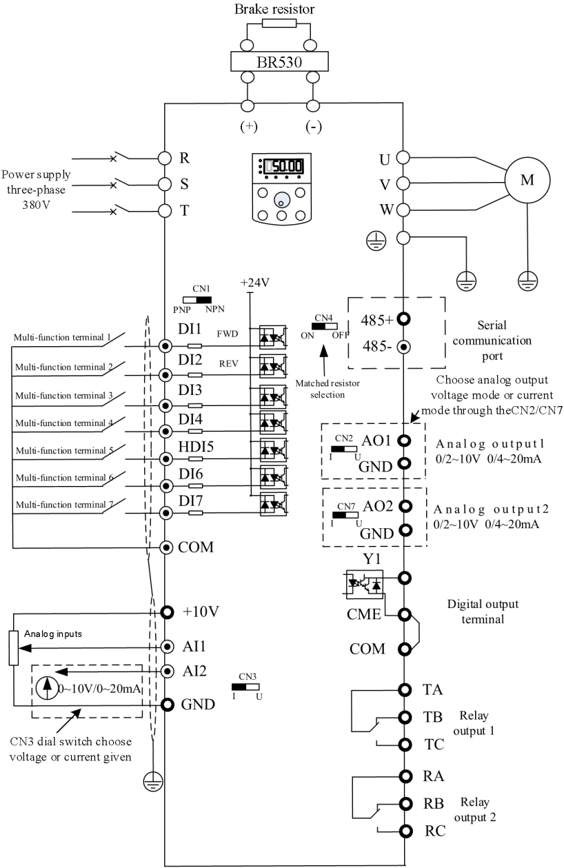
Fig.2-3 three-phase inverter within 30kW~55kW(380V/660V)
