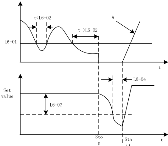
Fig.3-10 Sleep process frequency illustration
