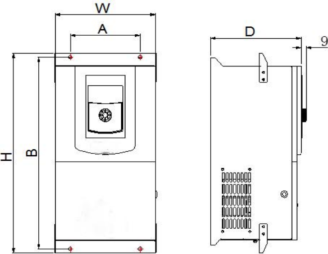
Fig1-2 Installation dimensions of metal mode 18~37kW
