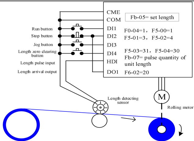
Fig.3-15 Examples of fixed-length control function
