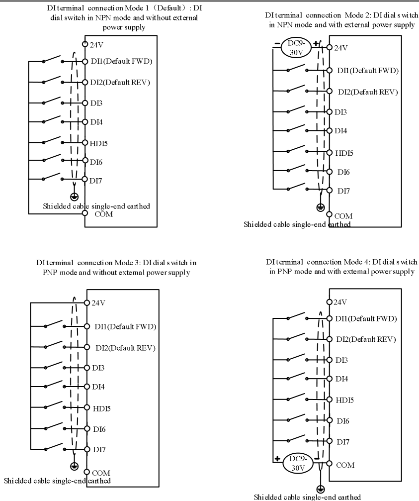
Fig 2-6 Four different wiring diagram
