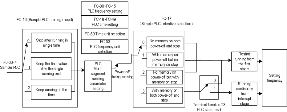
Fig.3-8 Sample PLC Illustration
