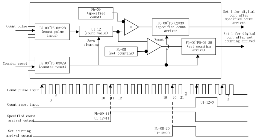
Fig.3-13 Counting mode function code setting
