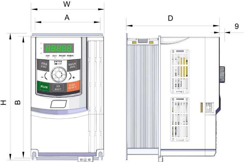
Fig.1-1 Installation dimensions of plastic mode below 15 kW
