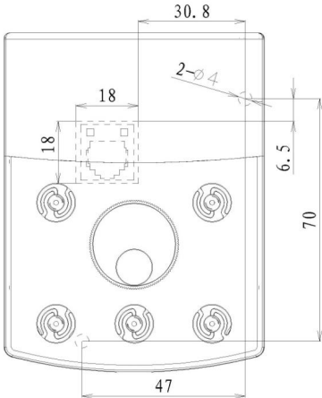
Fig.1-6 outer keyboard without plate installation dimension
