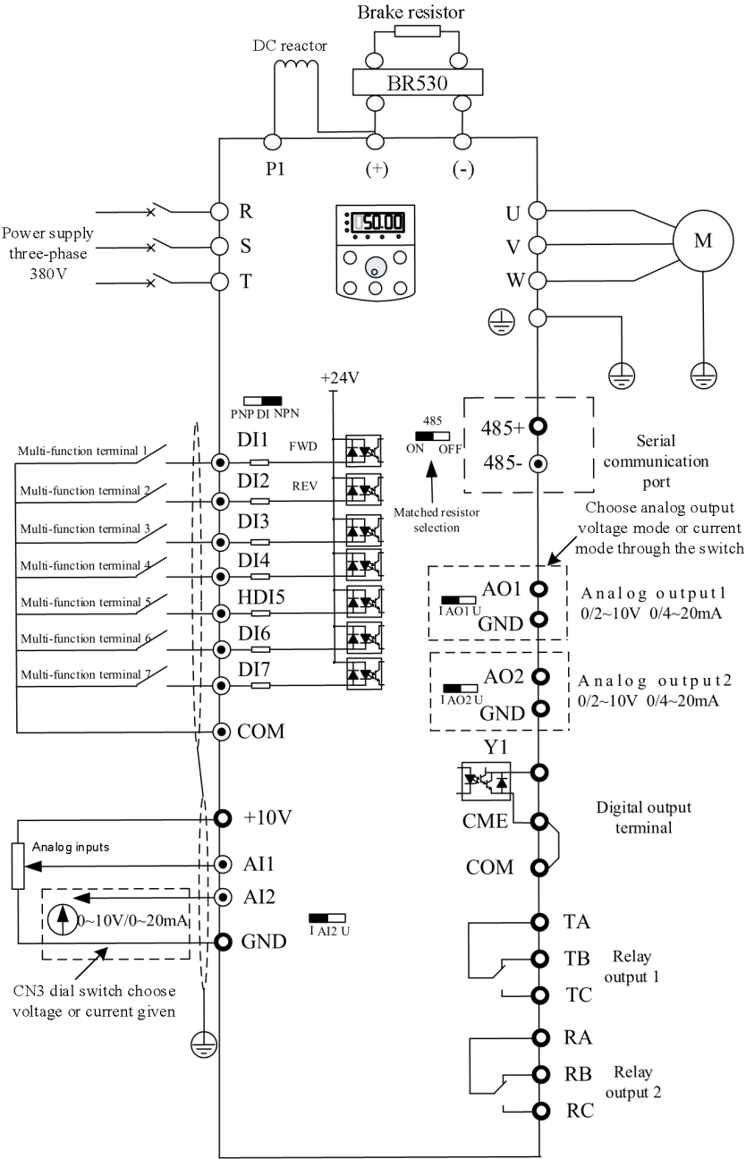
Fig.2-4 three-phase inverter above 75kW(380V/660V)
