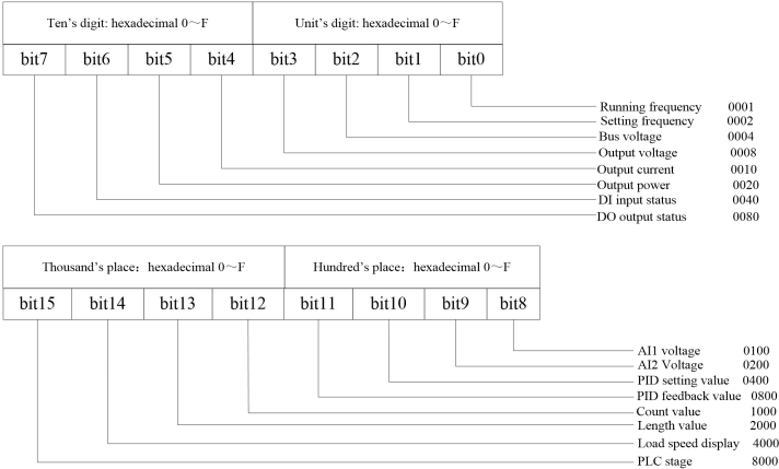
Fig.3-17 LED running display1 F7-29 illustration
