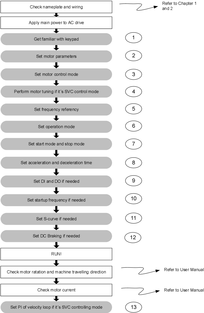
SetupFlowchart
