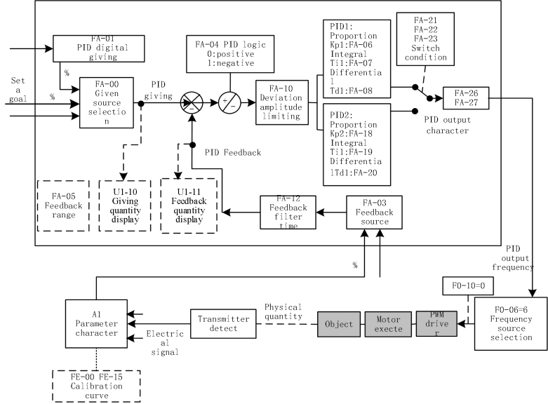
Fig.3-9 Illustration of frequency closed-loop control
